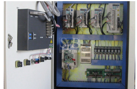
Control drives
